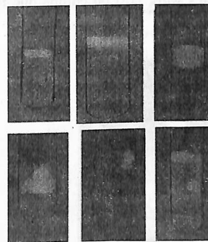
Figure 2. Change of chromatic pattern in Christiansen cell illuminated with laser with the passage of time.(after 10 sec , after 1 hours, after 6 hours , 10 hours, 22 hours, 48hours)
