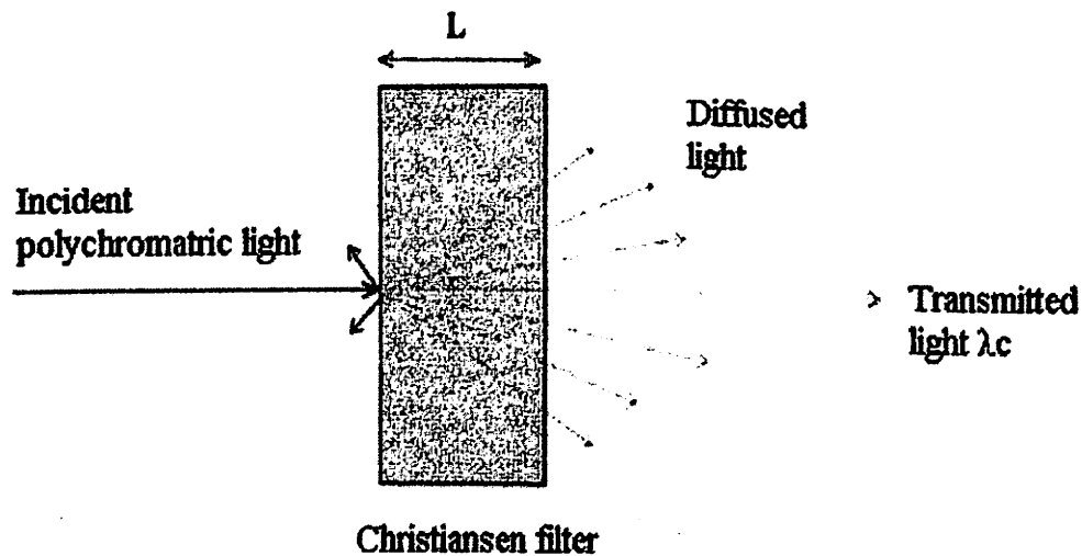
Figure 1: The Christiansen filtering: close to the wavelength \lambda_c for which refractive indexes of solid n_s and of liquid n_l match, light is transmitted. Other wavelengths are dispersed inside the cavity
