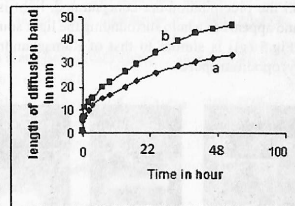
Figure 3: Diffusion band between CS 2 and acetone (a) with glass sphere, (b) with colloidal sample.
